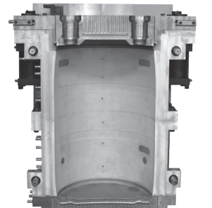
200L双口L环桶模具 200L Double L ring bucket mold
