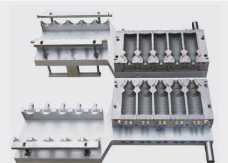
800ML五腔去飞边模具 800ML five-cavity deflashing mold
