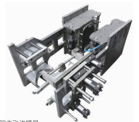
5L单腔去飞边模具 5L single cavity to deflashing mold
